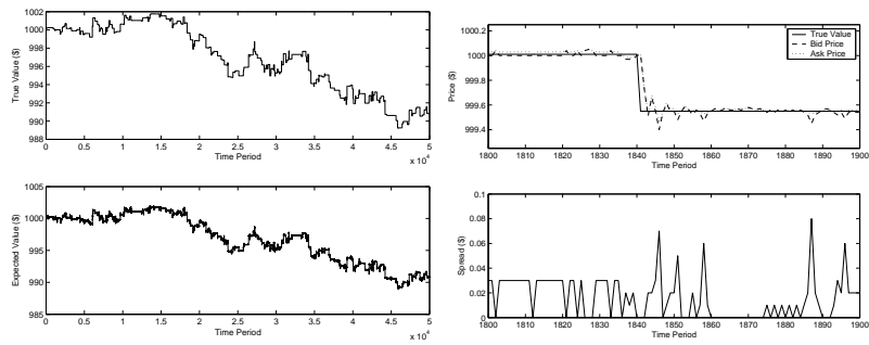
Figure 2.4: The market-maker's tracking of the true price over the course of the simulation (left) and immediately before and after a price jump (right)
