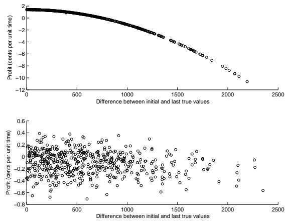
Figure 3.2: Naive market-maker profits as a function of market volatility without (above) and with (below) inventory control
