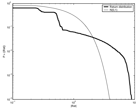
Figure 3.7: Leptokurtic distribution of absolute standardized log returns
