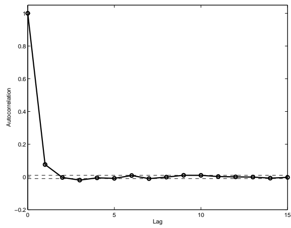
Figure 3.10: Autocorrelation of raw returns
