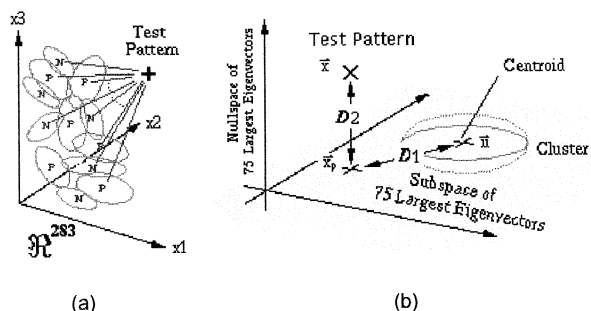
Fig. 4. Matching a test pattern against our distribution-based model. (a) Each set of measurements is a vector of 12 distances between the test pattern and the model’s 12 cluster centroids. (b) Each distance measurement between the test pattern and a cluster centroid is a two-value distance metric. D_1 is a Mahalanobis distance between the test pattern’s projection and the cluster centroid in a subspace spanned by the cluster’s 75 largest eigenvectors. D_2 is the Euclidean distance between the test pattern and its projection in the subspace.
