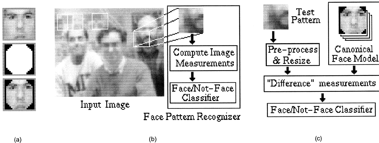
Fig. 1. Overview of our face-detection system. (a) A "canonical" face pattern, a 19 \times 19 mask for eliminating near-boundary pixels of canonical face patterns, and the resulting "canonical" face pattern after applying the mask. (b) At each scale, the image is divided into many possibly overlapping windows. Each window pattern gets classified as either "a face" or "not a face," based on a set of local image measurements. (c) The key components of the Face Pattern Recognizer block in greater detail.
